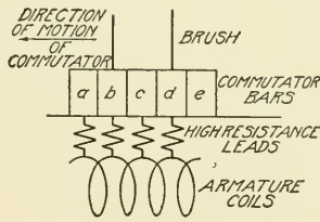
Fig. 51. High-Resistance Commutator Leads
